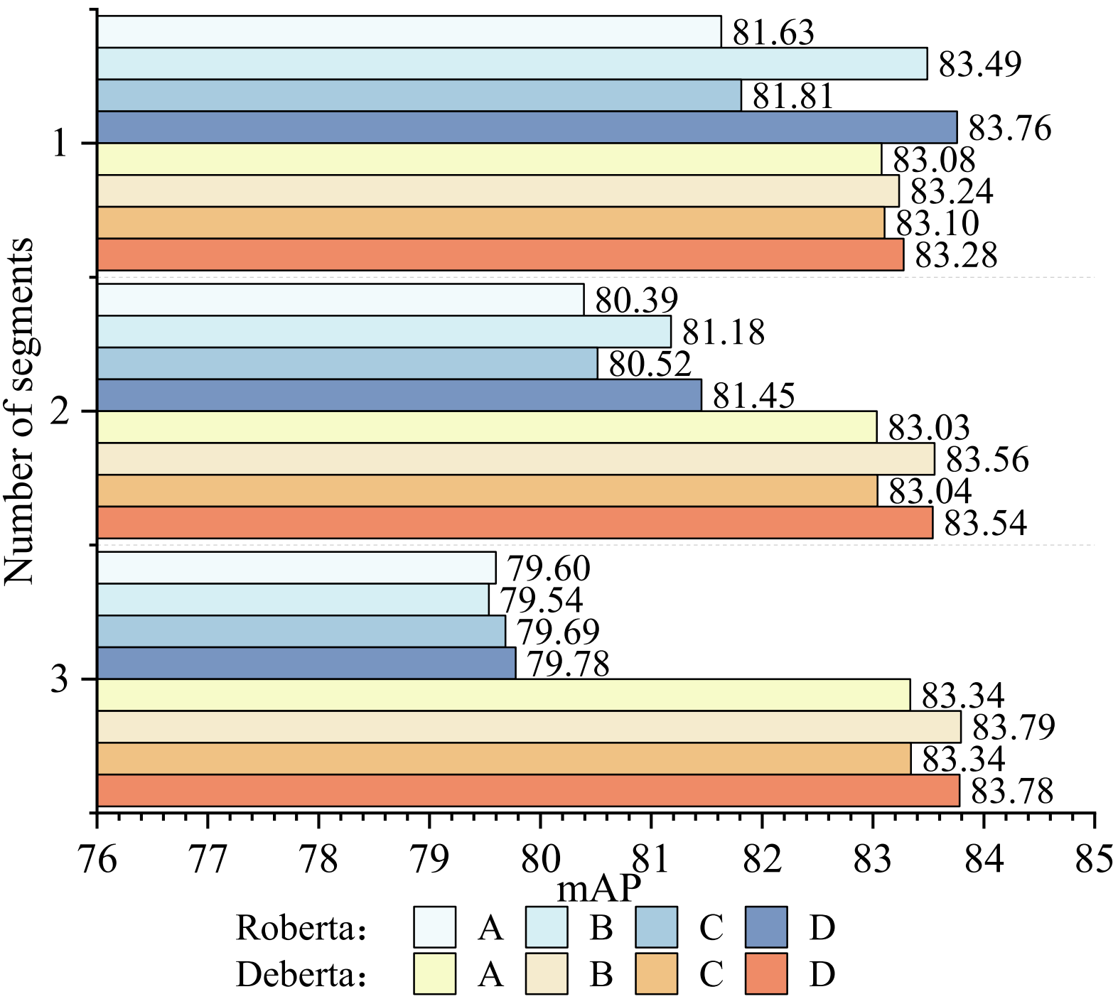
mAP on GoodNews
